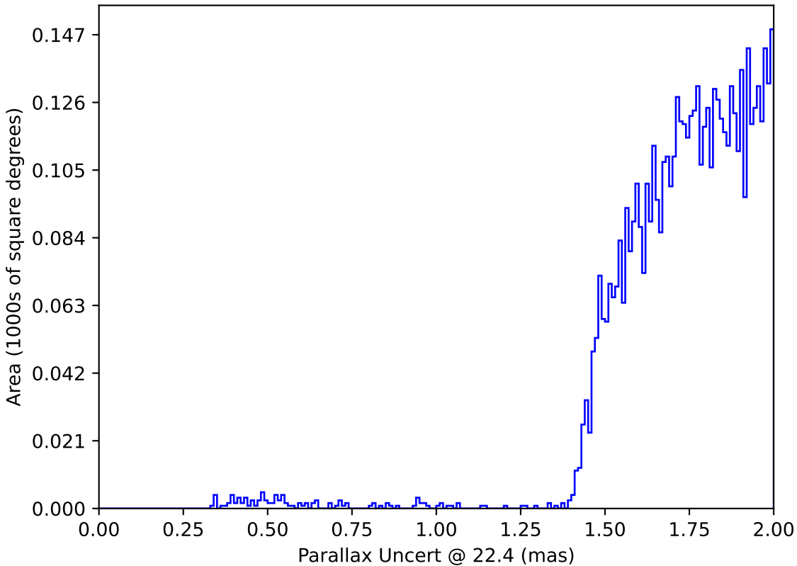
weather_cloudso30v3.4_10yrs : Parallax Uncert @ 22.4
