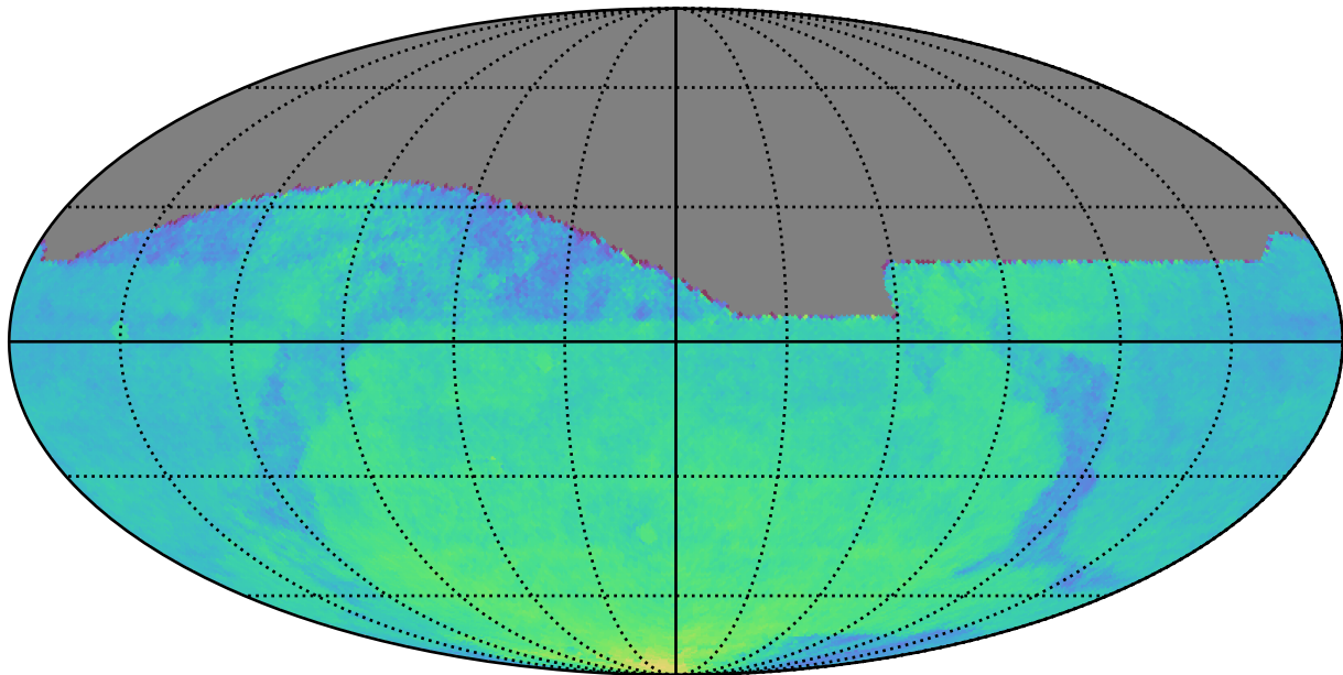
weather_cloudso30v3.4_10yrs : Parallax Coverage @ 22.4
