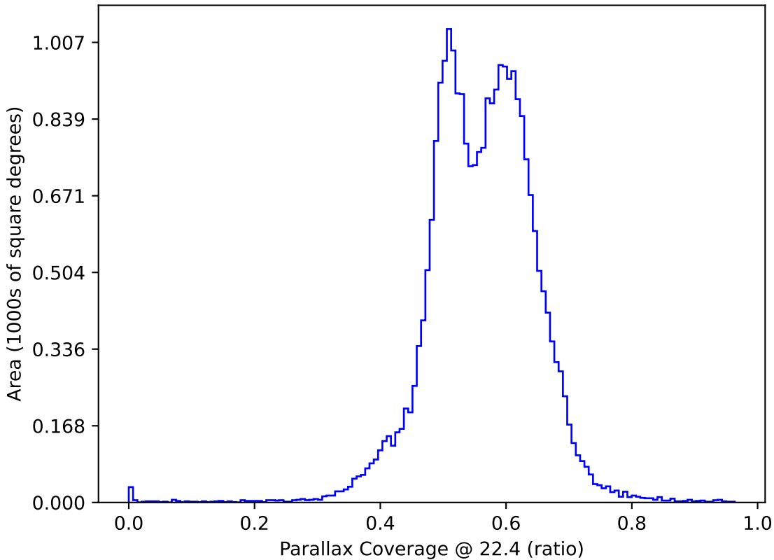
weather_cloudso30v3.4_10yrs : Parallax Coverage @ 22.4
