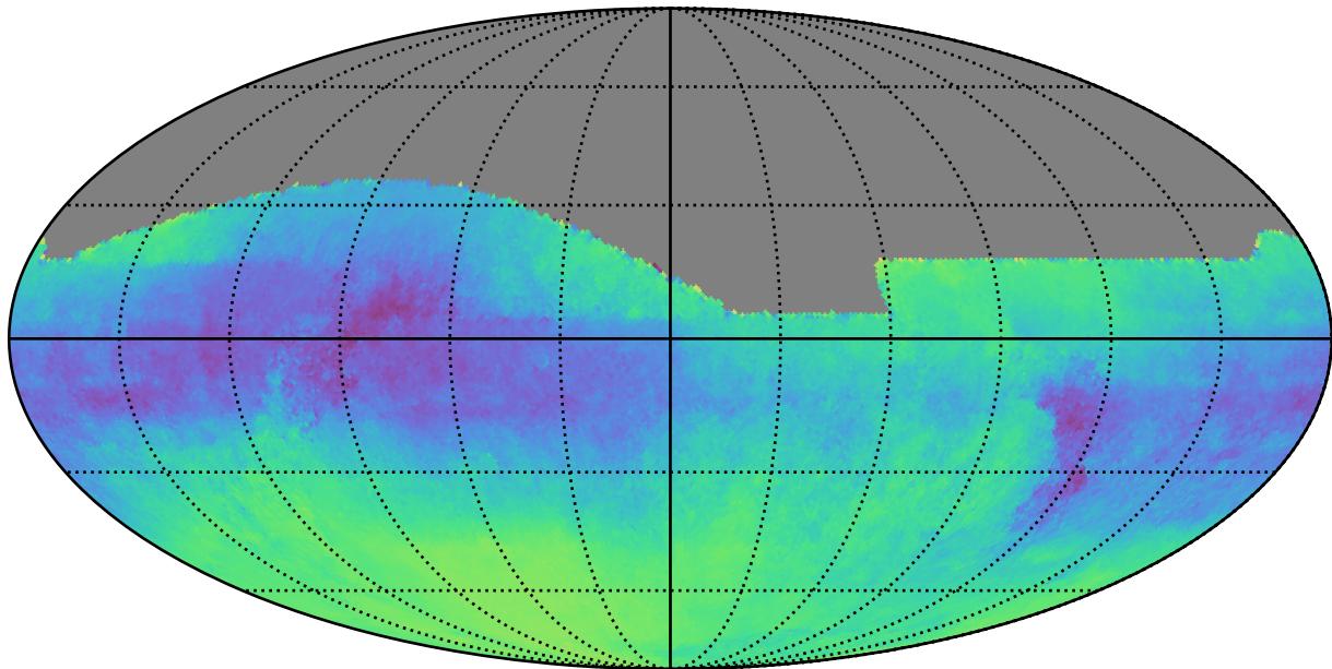
weather_cloudso30v3.4_10yrs : Parallax-DCR degeneracy @ 24.0
