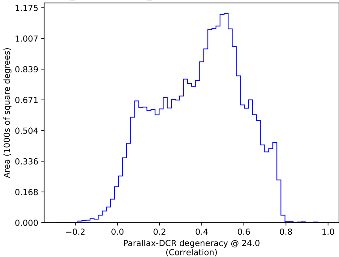
weather_cloudso30v3.4_10yrs : Parallax-DCR degeneracy @ 24.0
