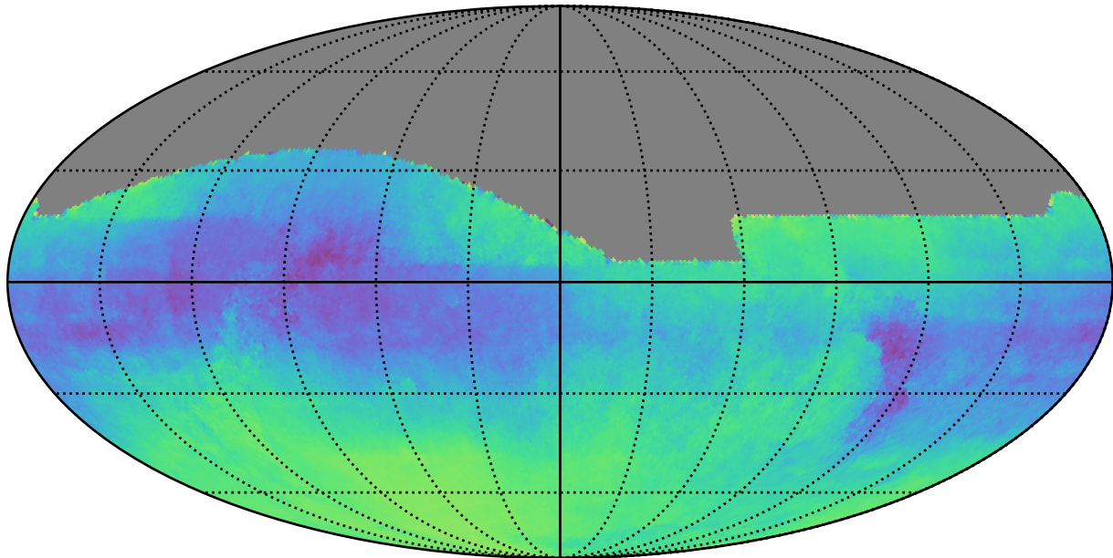
weather_cloudso30v3.4_10yrs : Parallax-DCR degeneracy @ 22.4
