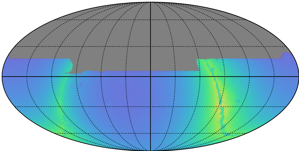
weather_cloudso30v3.4_10yrs y: Nstars_no_crowding
