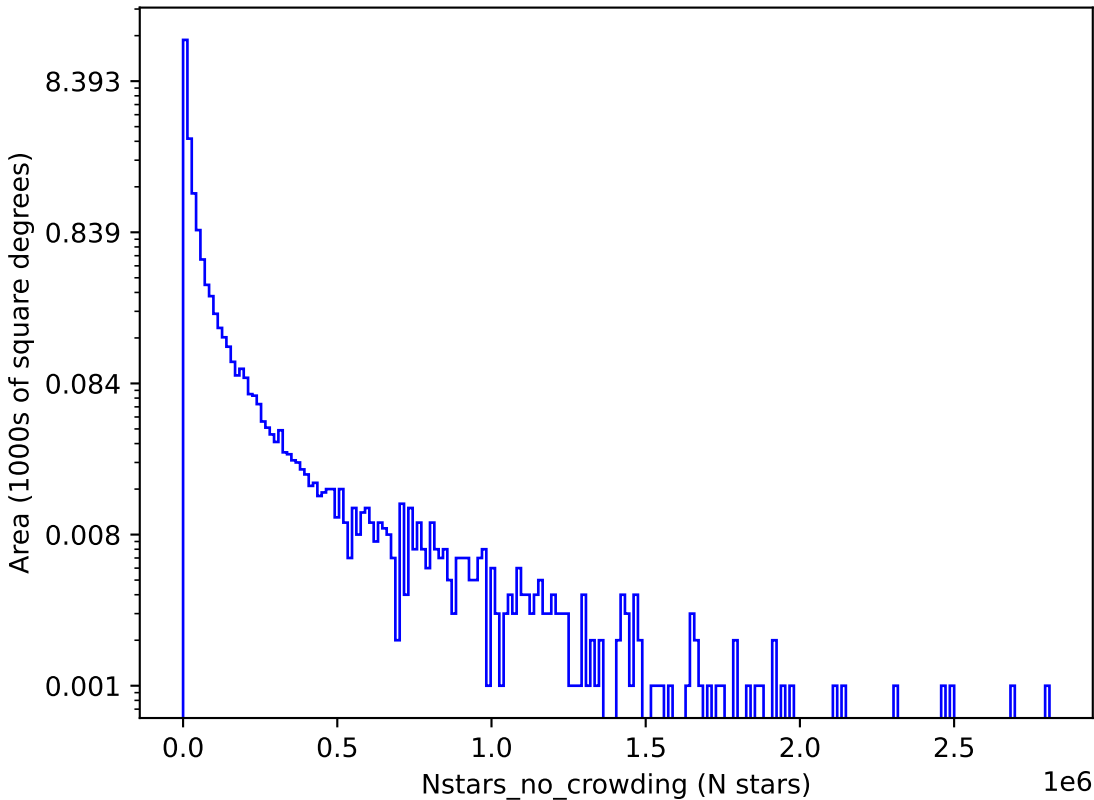
weather_cloudso30v3.4_10yrs u: Nstars_no_crowding
