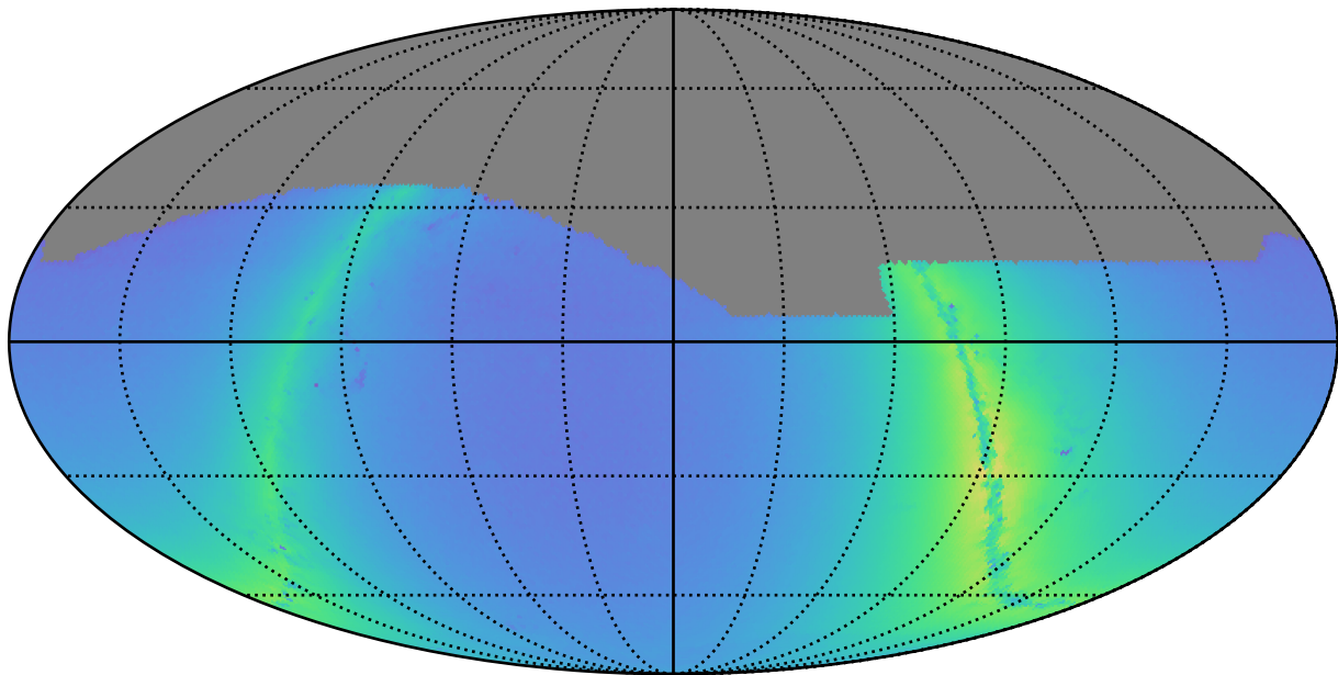
weather_cloudso30v3.4_10yrs r: Nstars_no_crowding
