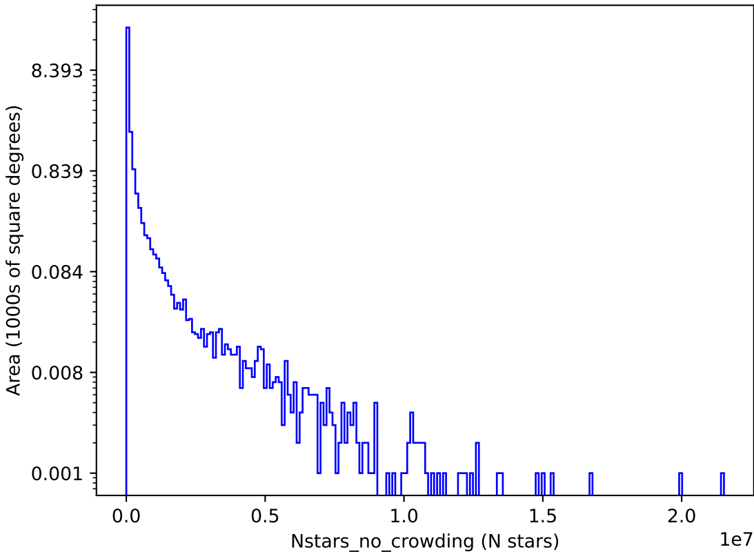
weather_cloudso30v3.4_10yrs r: Nstars_no_crowding
