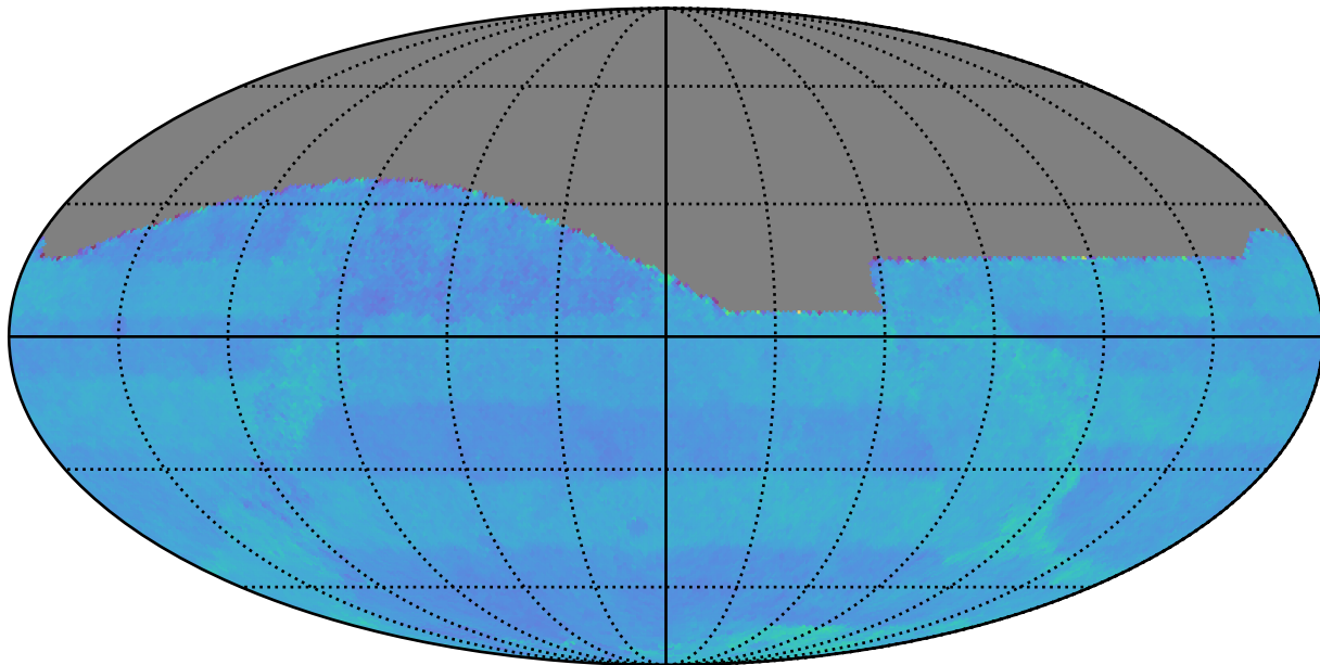
weather_cloudso30v3.4_10yrs : Normalized Proper Motion Uncert @ 24.0
