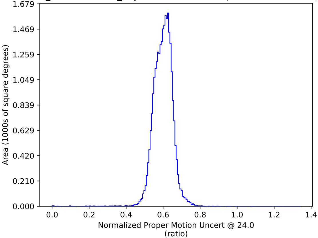
weather_cloudso30v3.4_10yrs : Normalized Proper Motion Uncert @ 24.0
