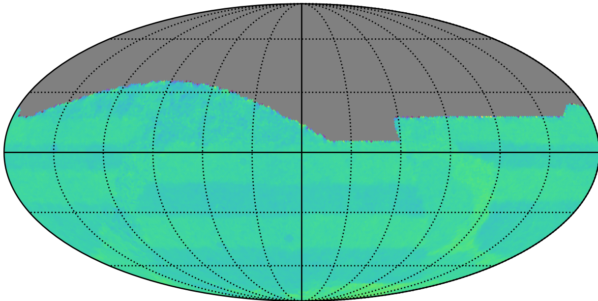
weather_cloudso30v3.4_10yrs : Normalized Proper Motion Uncert @ 20.5
