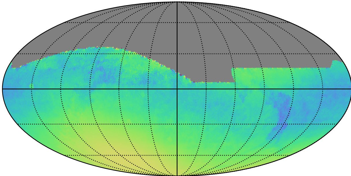
weather_cloudso30v3.4_10yrs : Normalized Parallax Uncert @ 24.0
