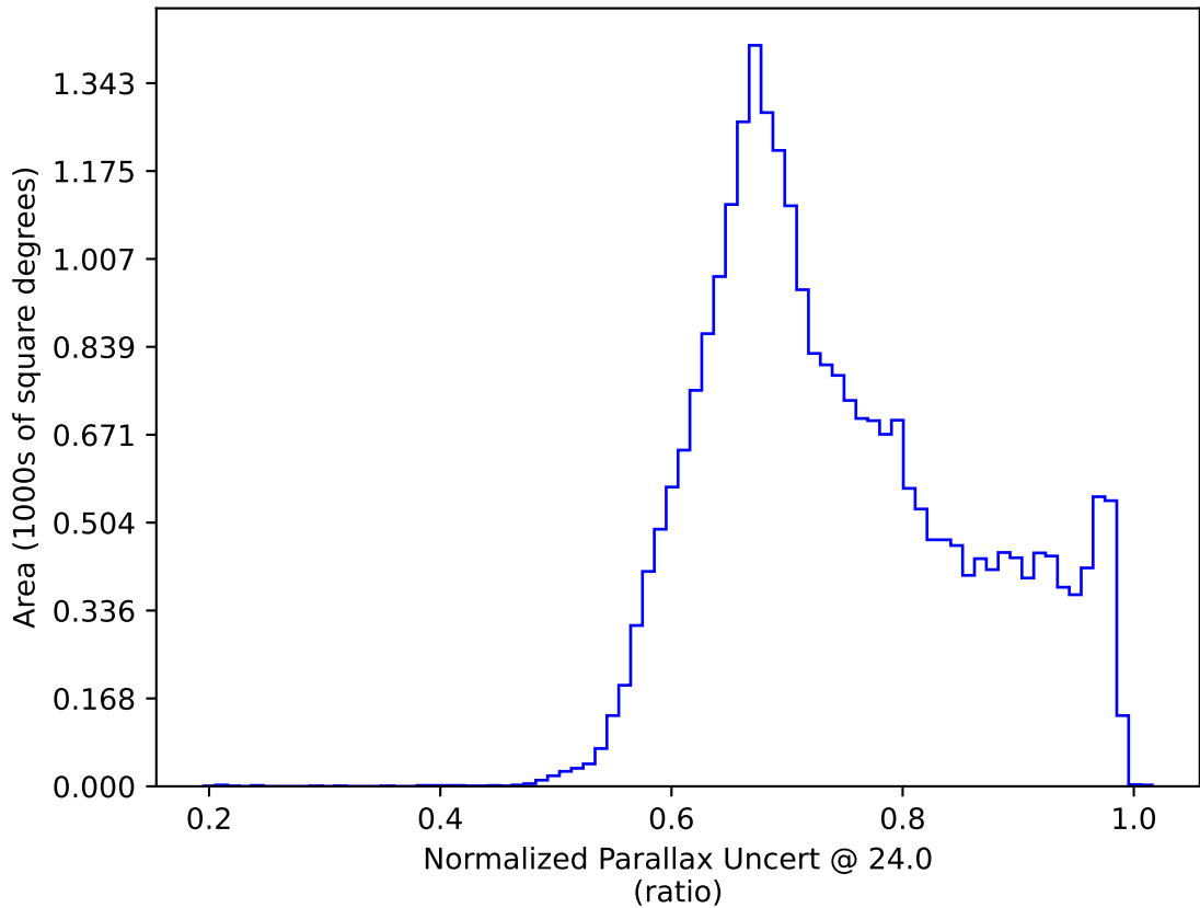
weather_cloudso30v3.4_10yrs : Normalized Parallax Uncert @ 24.0
