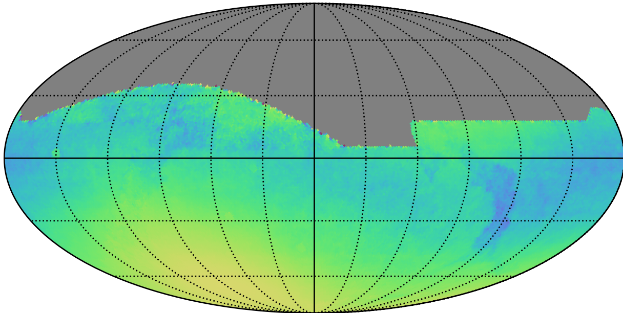
weather_cloudso30v3.4_10yrs : Normalized Parallax Uncert @ 22.4
