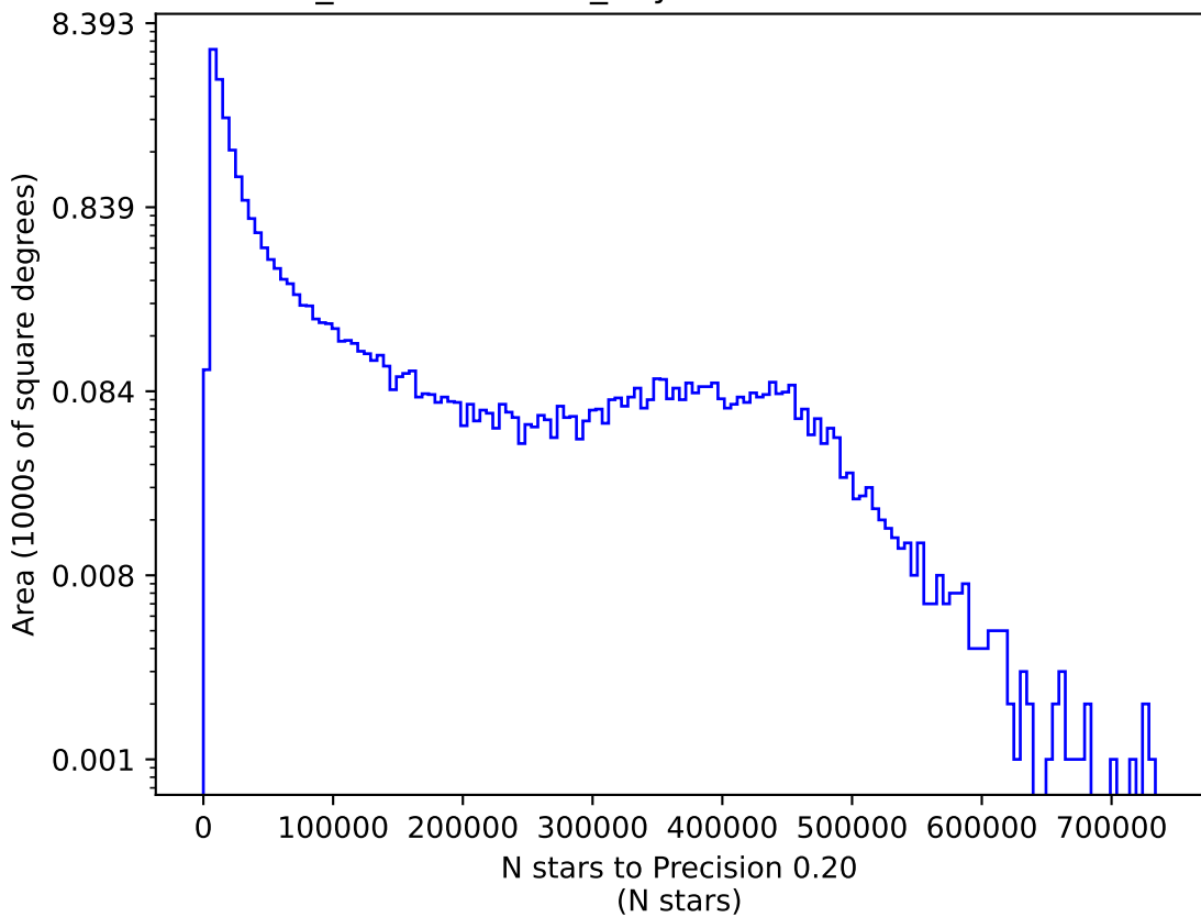
weather_cloudso30v3.4_10yrs z: N stars to Precision 0.20
