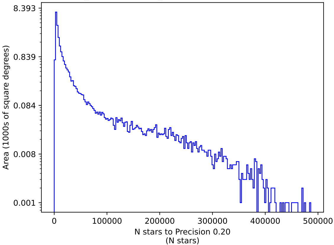
weather_cloudso30v3.4_10yrs u: N stars to Precision 0.20
