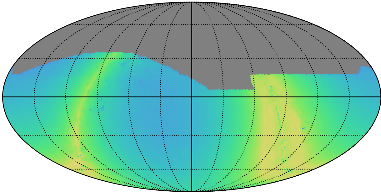
weather_cloudso30v3.4_10yrs r: N stars to Precision 0.20
