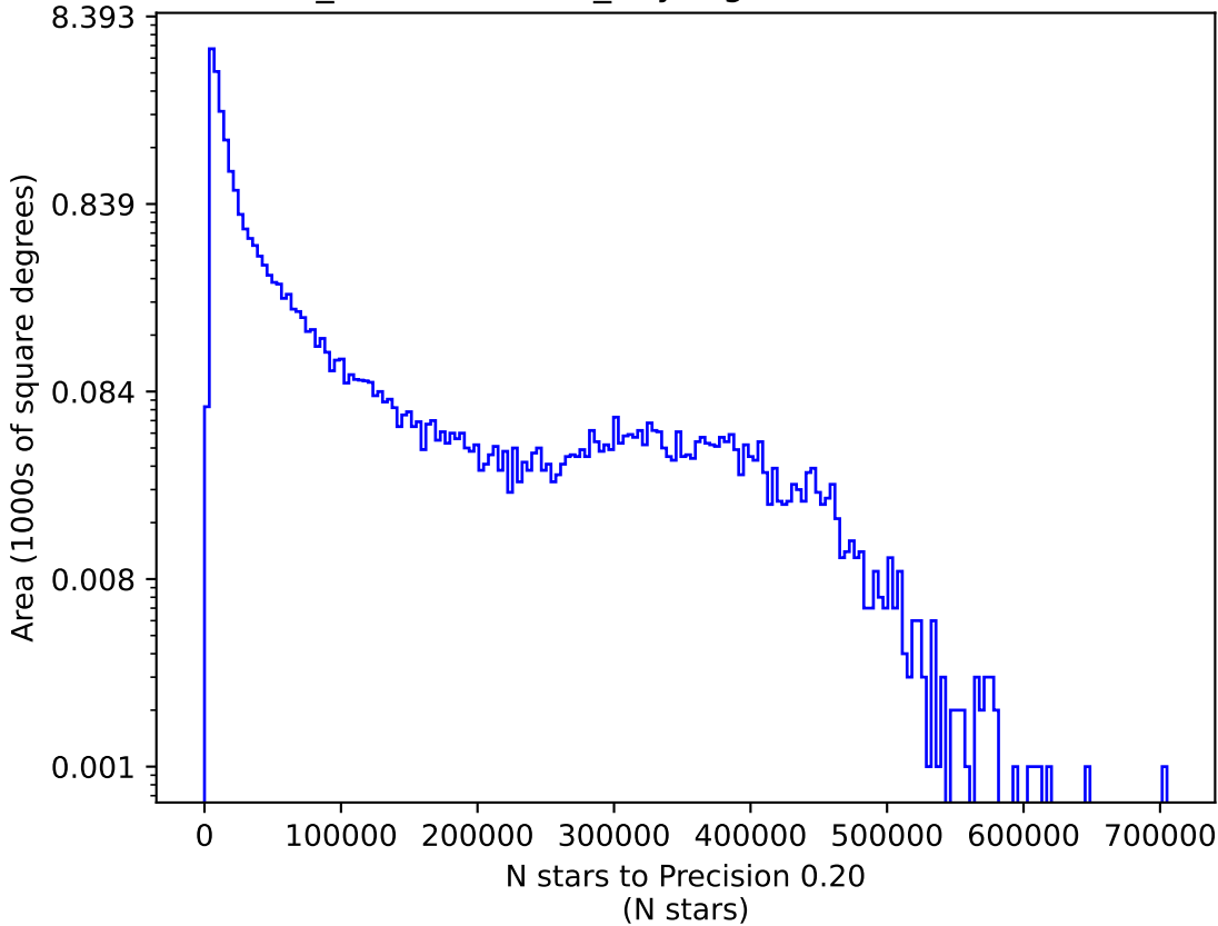
weather_cloudso30v3.4_10yrs g: N stars to Precision 0.20
