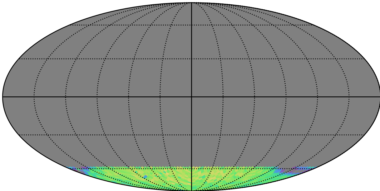
weather_cloudso30v3.4_10yrs gi SCP: LVDwarfs
