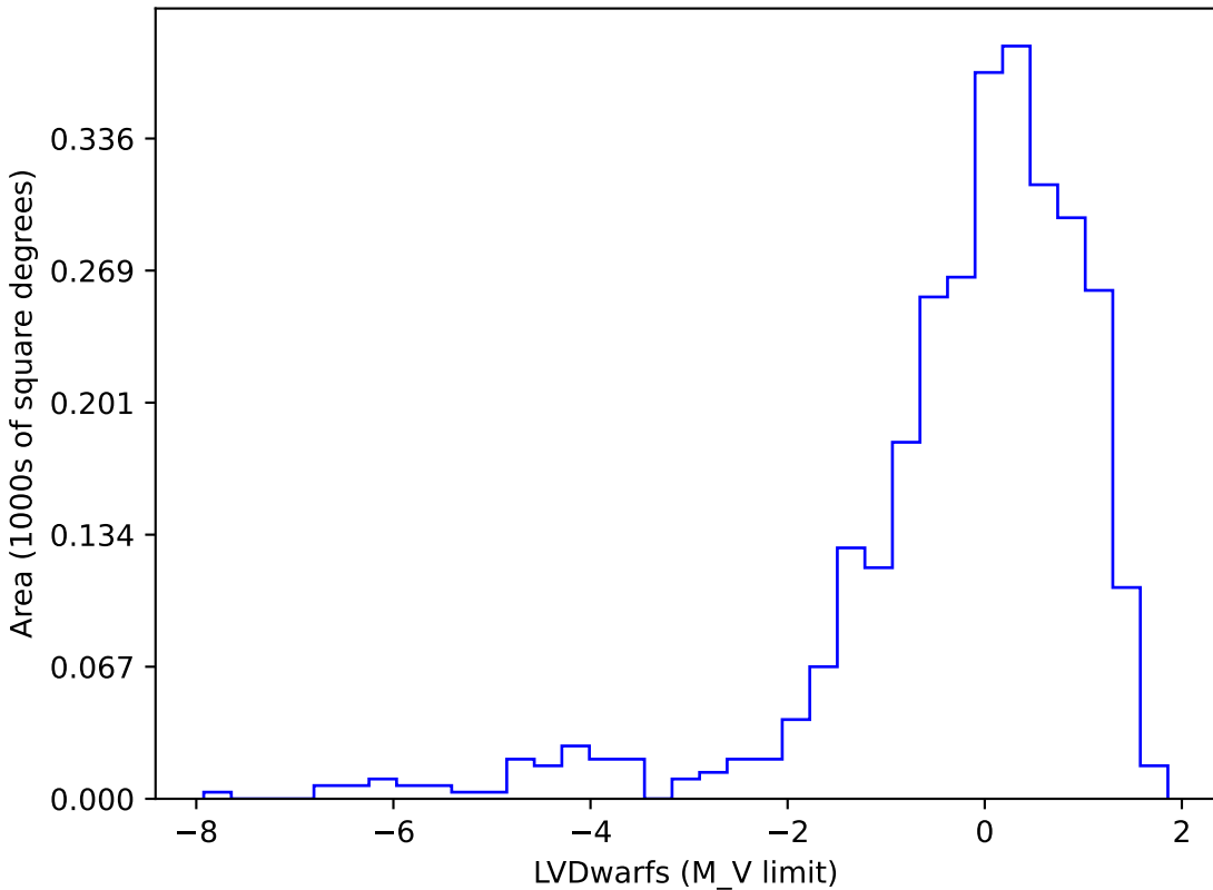
weather_cloudso30v3.4_10yrs gi SCP: LVDwarfs
