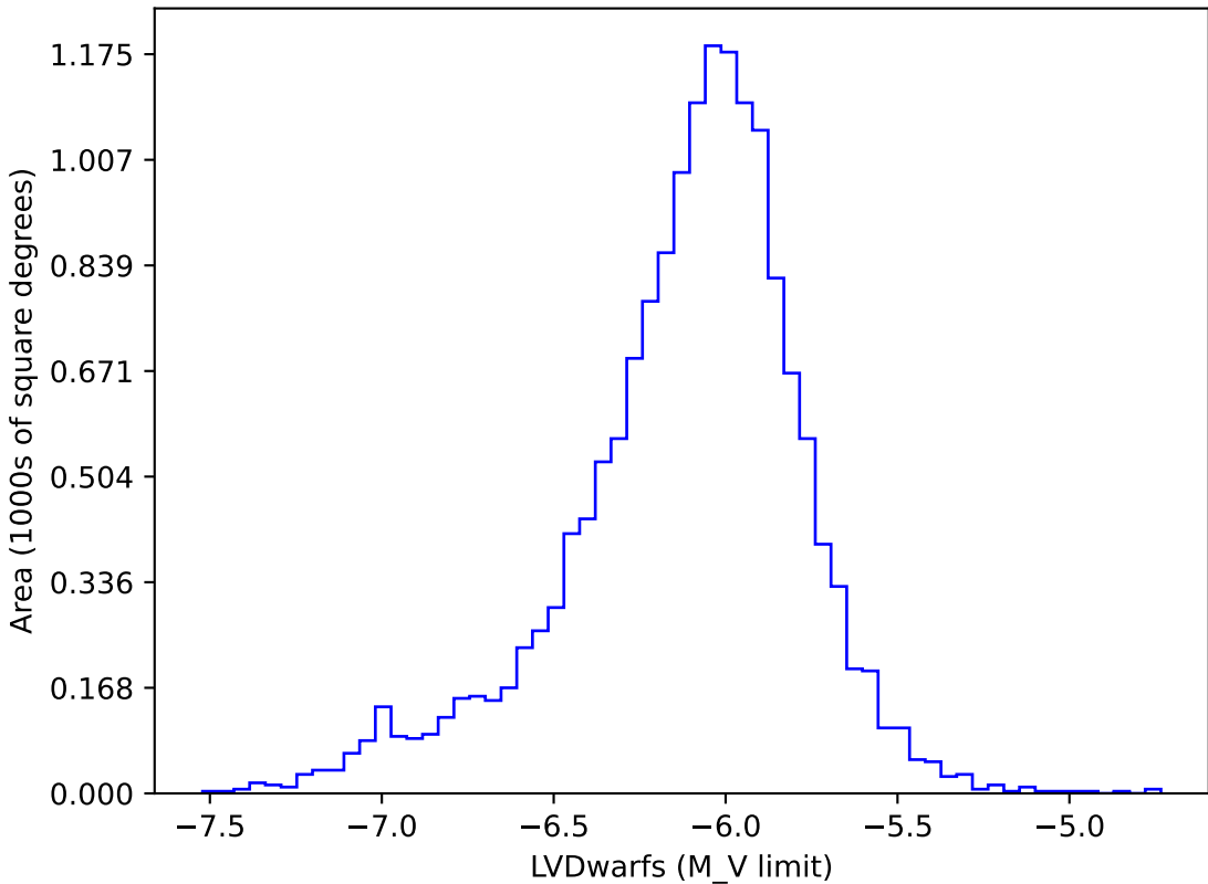
weather_cloudso30v3.4_10yrs gi: LVDwarfs
