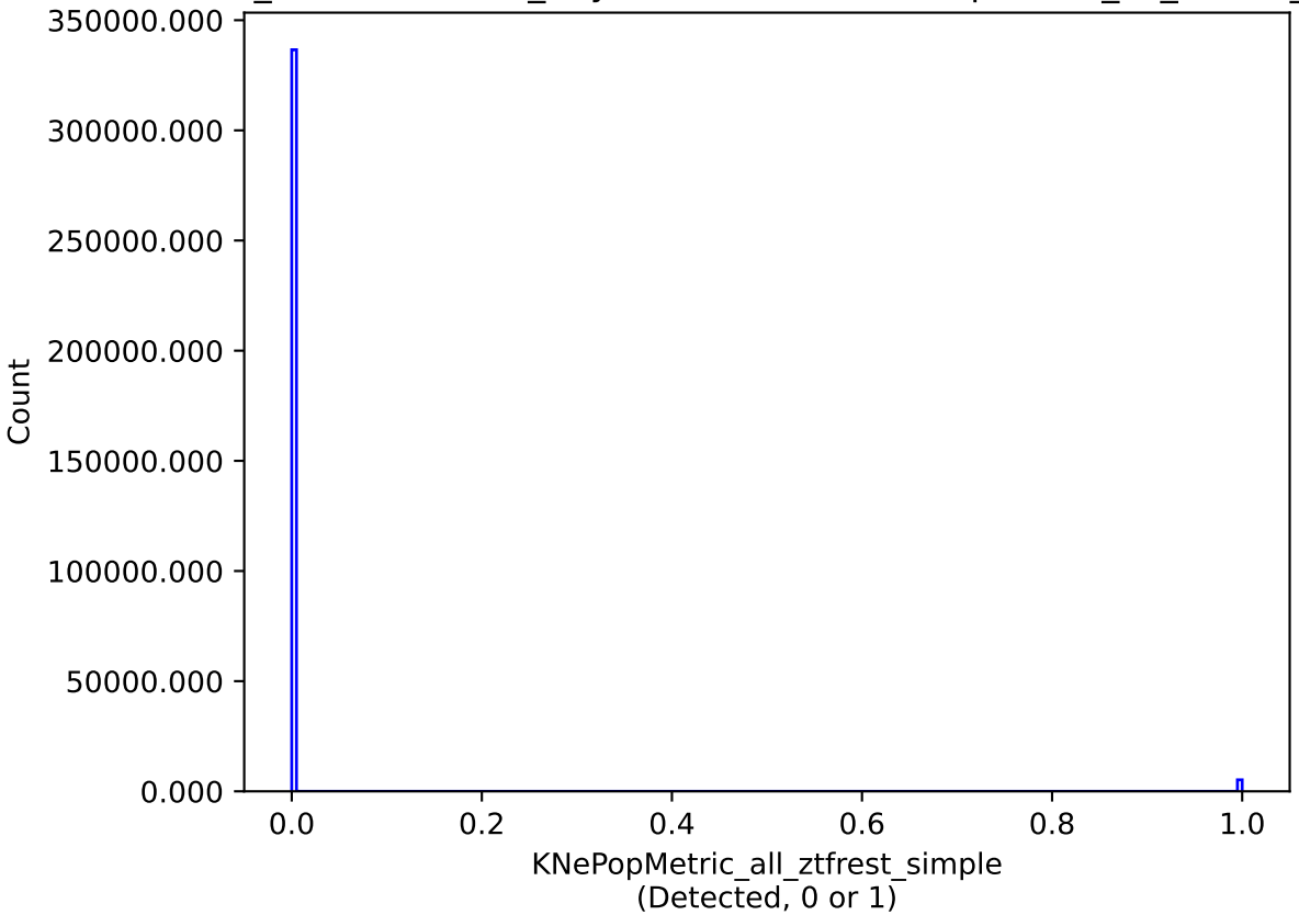
weather_cloudso30v3.4_10yrs all models: KNePopMetric_all_ztfrest_simple
