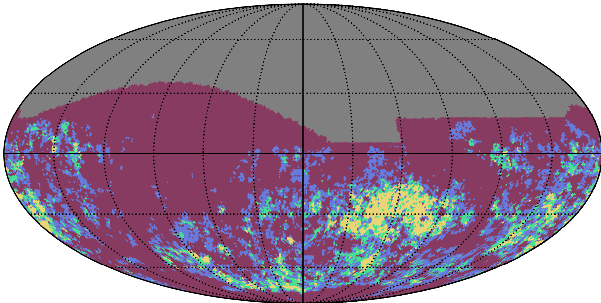
weather_cloudso30v3.4_10yrs z band: Gaps_7hr
