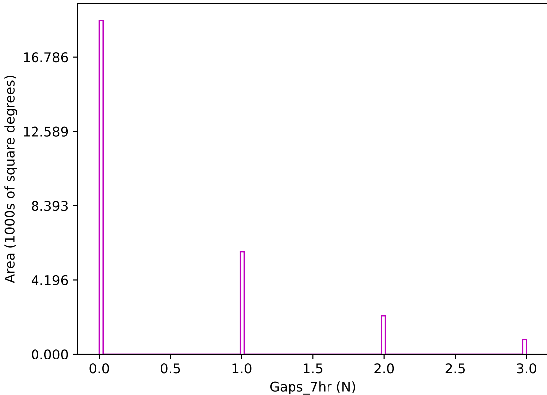
weather_cloudso30v3.4_10yrs z band: Gaps_7hr
