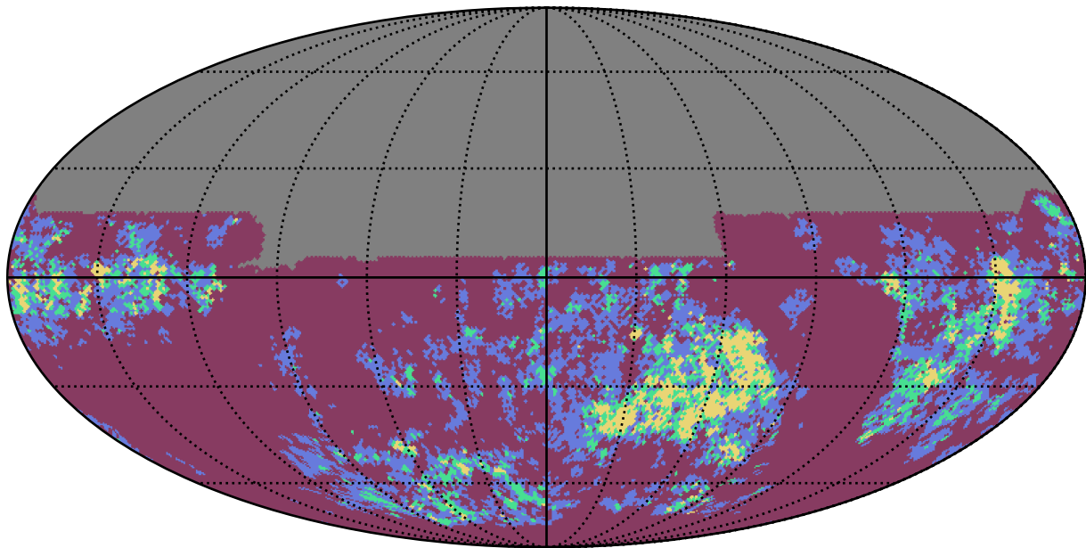
weather_cloudso30v3.4_10yrs y band: Gaps_7hr
