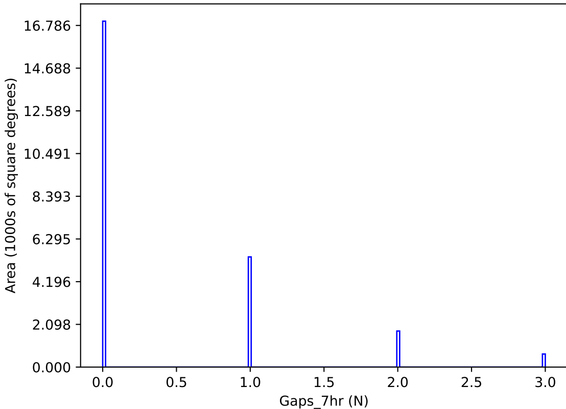
weather_cloudso30v3.4_10yrs y band: Gaps_7hr
