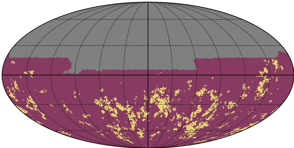
weather_cloudso30v3.4_10yrs u band: Gaps_7hr
