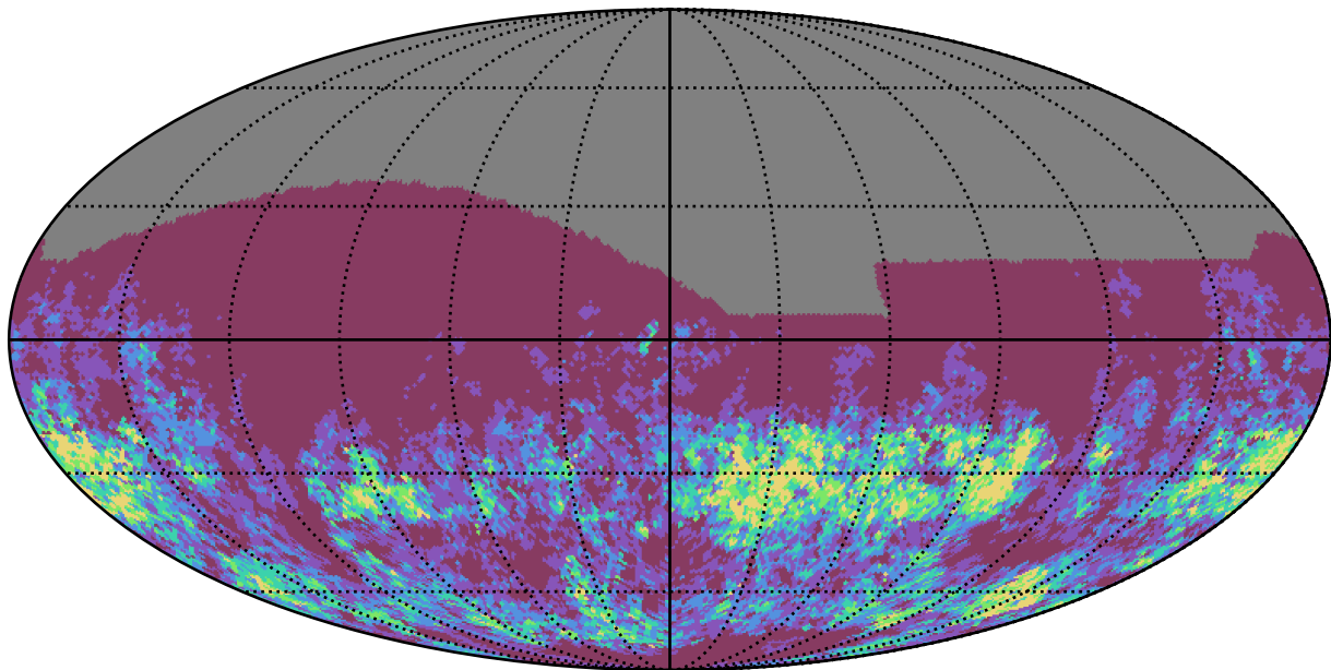
weather_cloudso30v3.4_10yrs r band: Gaps_7hr
