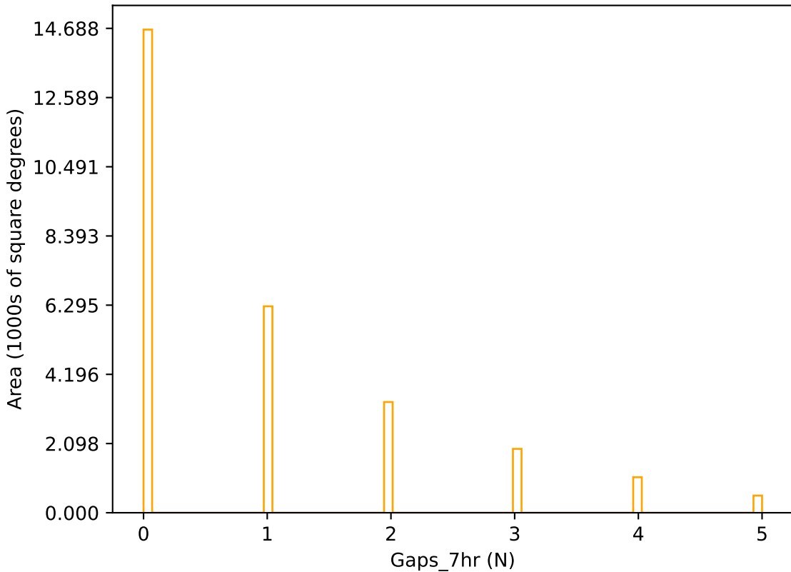
weather_cloudso30v3.4_10yrs r band: Gaps_7hr
