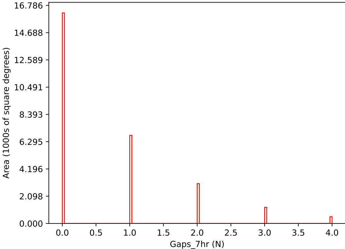
weather_cloudso30v3.4_10yrs i band: Gaps_7hr
