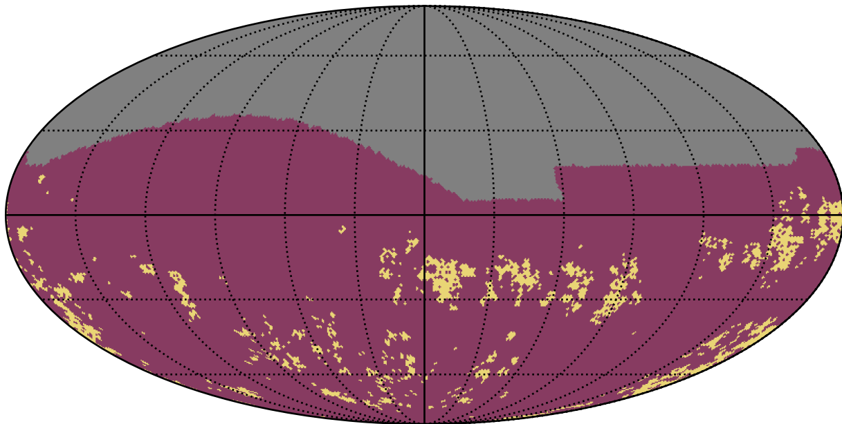
weather_cloudso30v3.4_10yrs g band: Gaps_7hr
