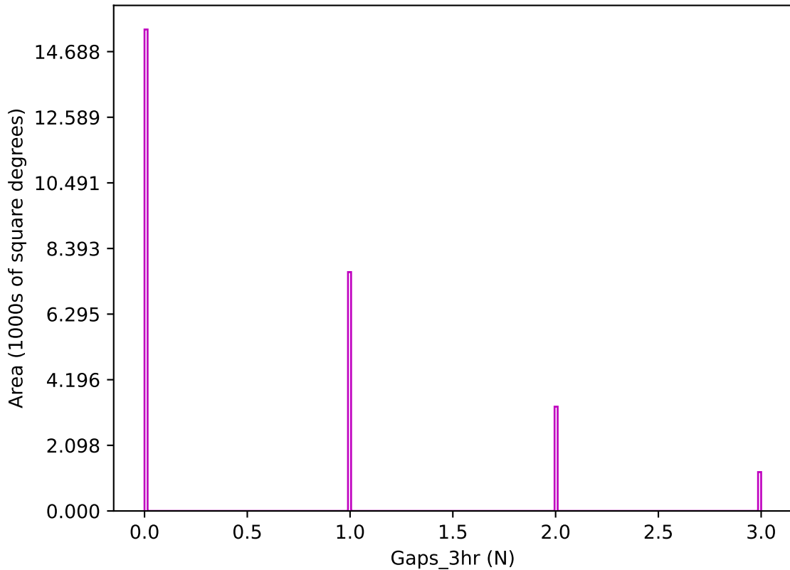
weather_cloudso30v3.4_10yrs z band: Gaps_3hr
