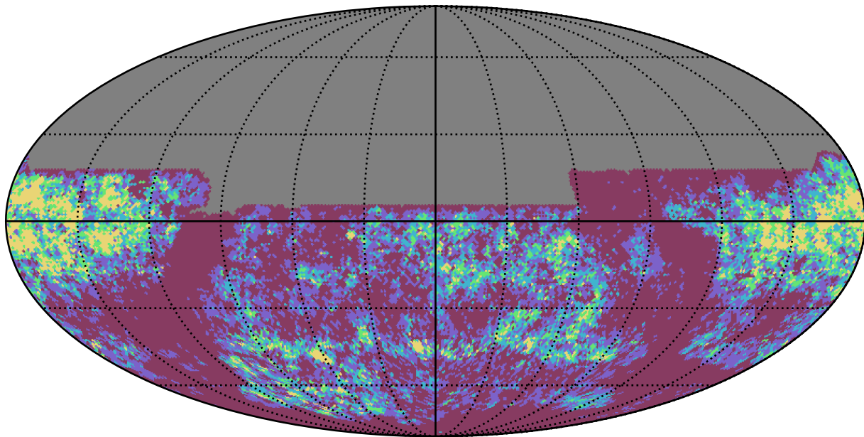
weather_cloudso30v3.4_10yrs y band: Gaps_3hr
