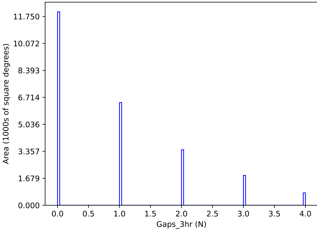
weather_cloudso30v3.4_10yrs y band: Gaps_3hr
