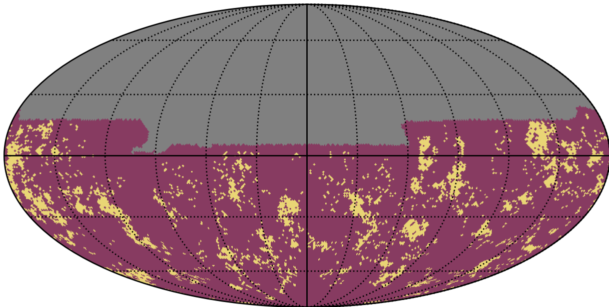
weather_cloudso30v3.4_10yrs u band: Gaps_3hr
