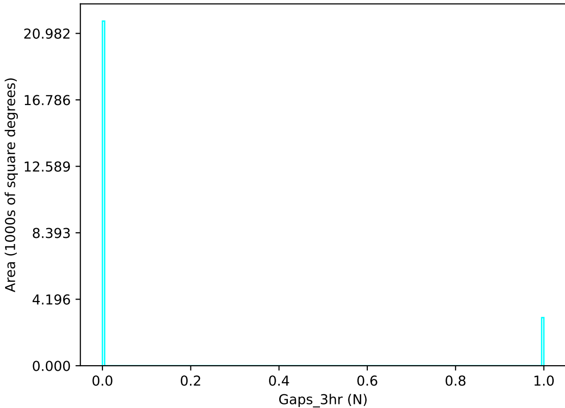
weather_cloudso30v3.4_10yrs u band: Gaps_3hr
