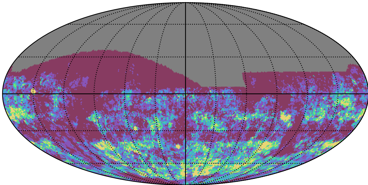
weather_cloudso30v3.4_10yrs r band: Gaps_3hr
