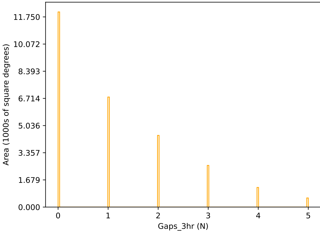
weather_cloudso30v3.4_10yrs r band: Gaps_3hr
