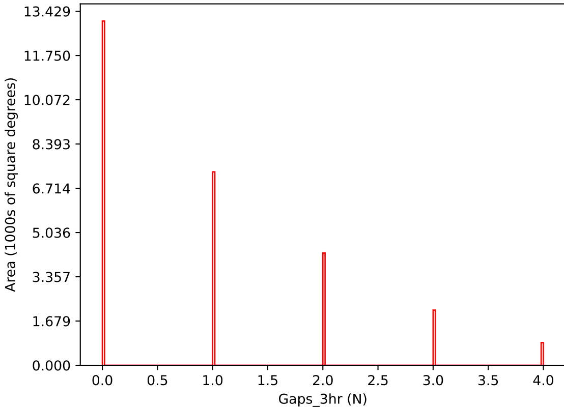
weather_cloudso30v3.4_10yrs i band: Gaps_3hr
