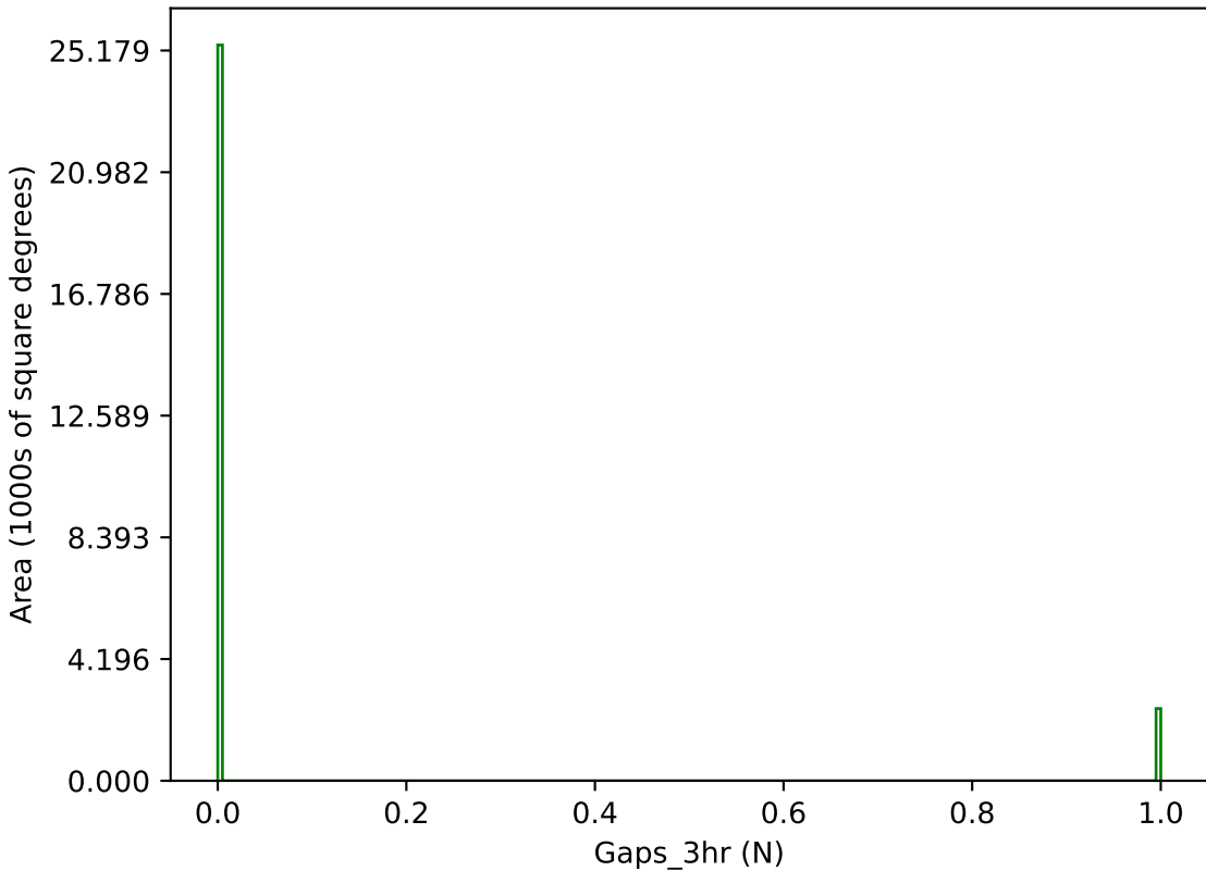
weather_cloudso30v3.4_10yrs g band: Gaps_3hr
