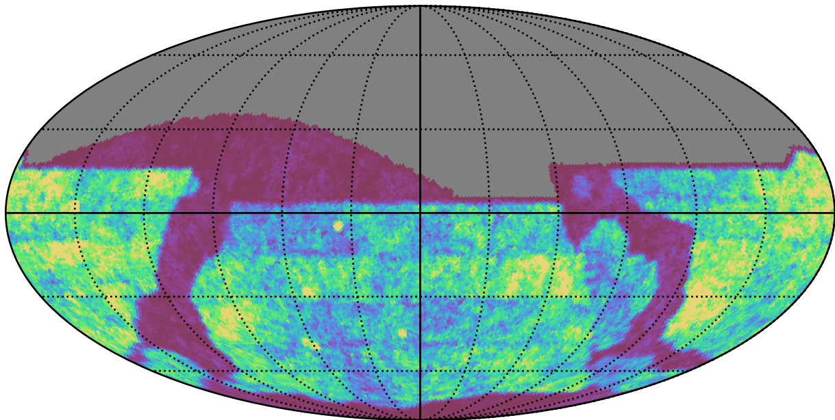
weather_cloudso30v3.4_10yrs z band: Gaps_24hr
