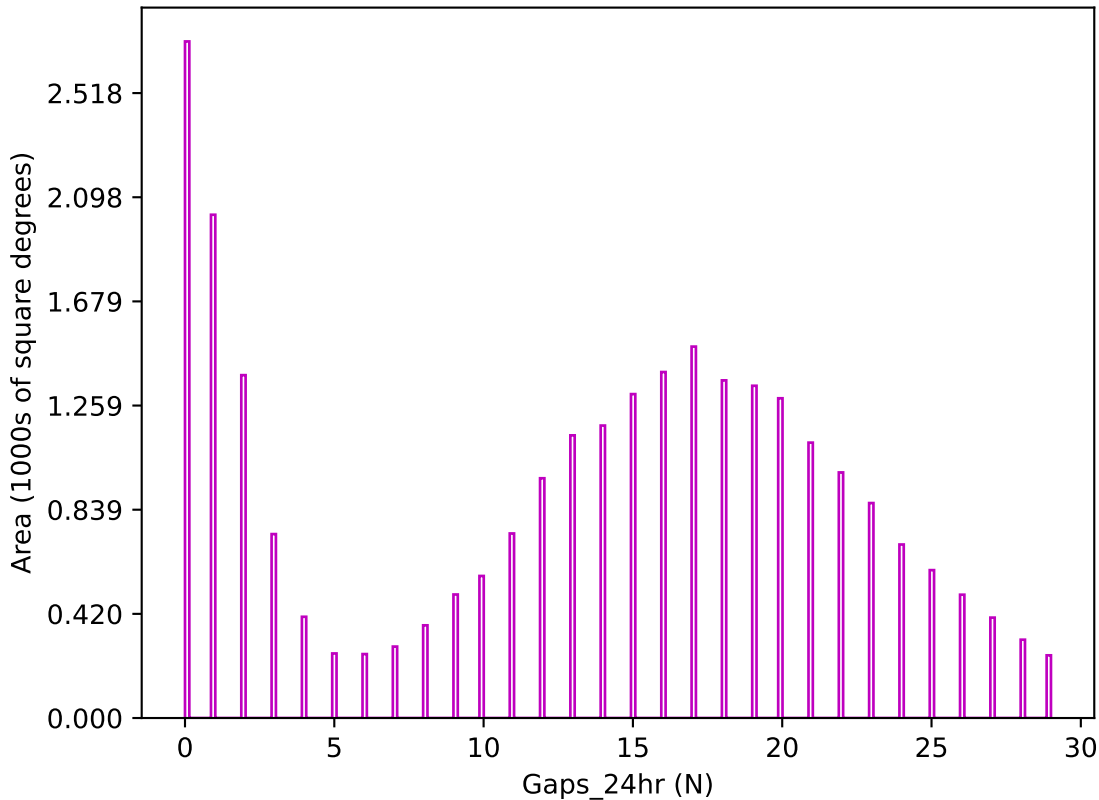
weather_cloudso30v3.4_10yrs z band: Gaps_24hr
