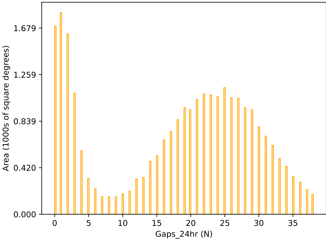
weather_cloudso30v3.4_10yrs r band: Gaps_24hr
