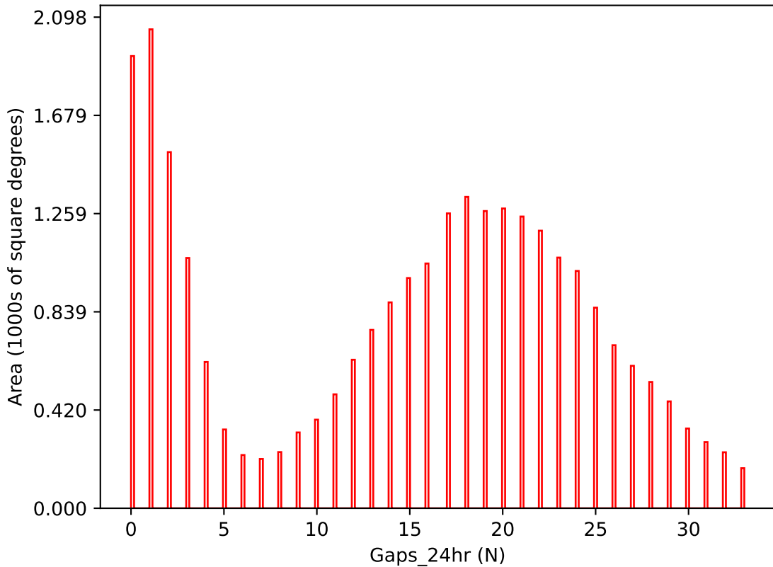
weather_cloudso30v3.4_10yrs i band: Gaps_24hr
