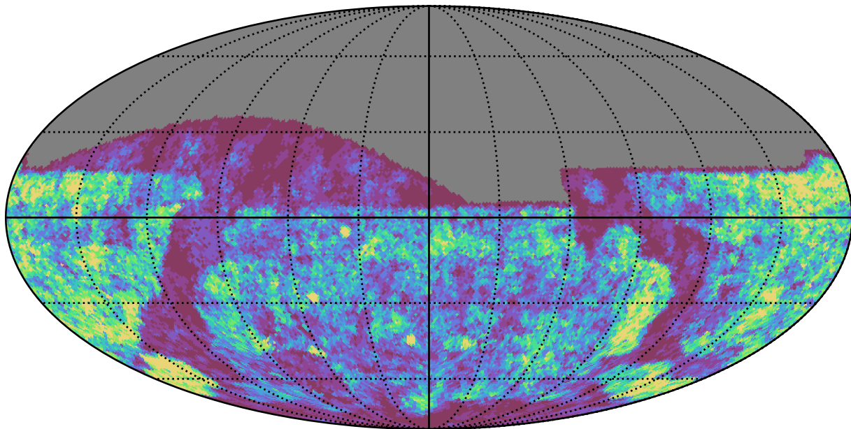
weather_cloudso30v3.4_10yrs g band: Gaps_24hr
