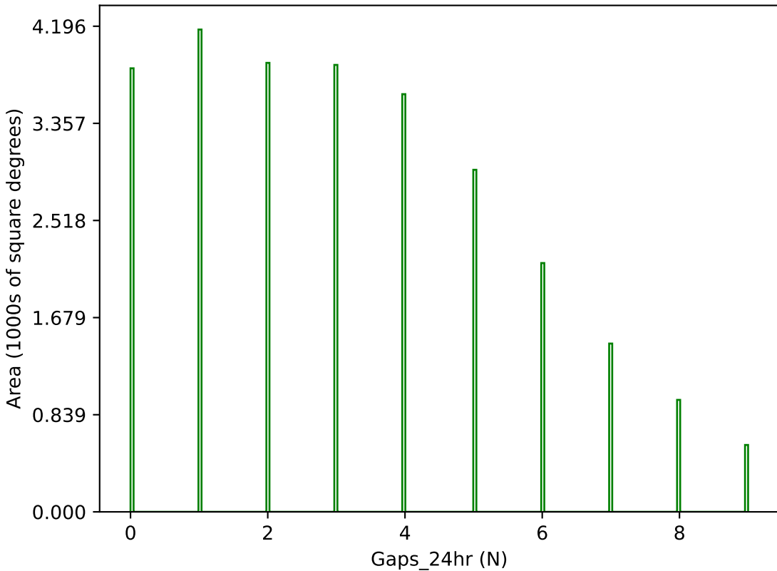
weather_cloudso30v3.4_10yrs g band: Gaps_24hr
