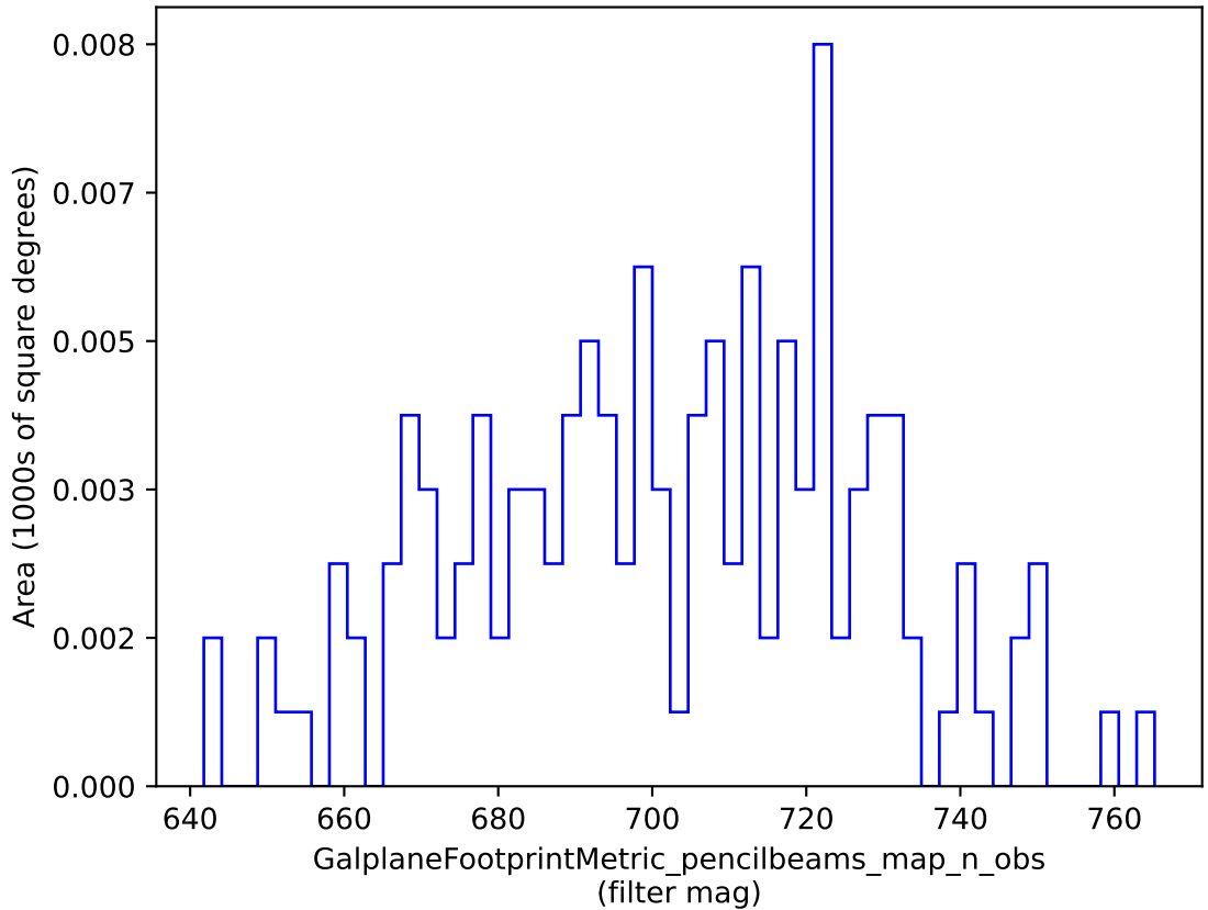
weather_cloudso30v3.4_10yrs : GalplaneFootprintMetric_pencilbeams_map_n_obs
