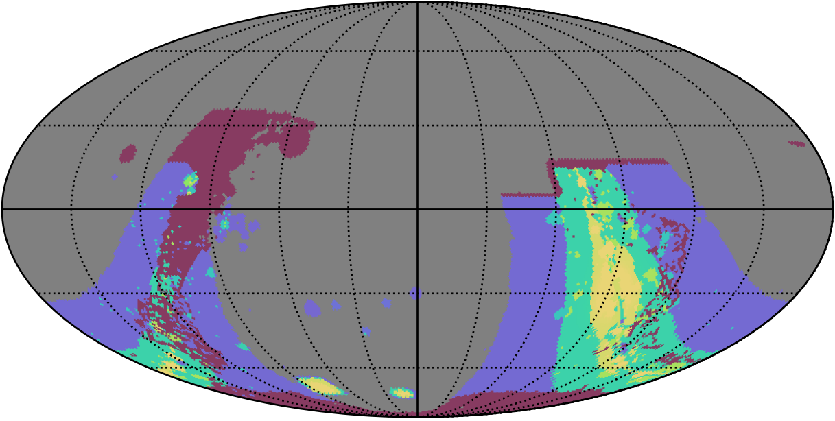
weather_cloudso30v3.4_10yrs : GalplaneFootprintMetric_combined_map_Tau_20_0
